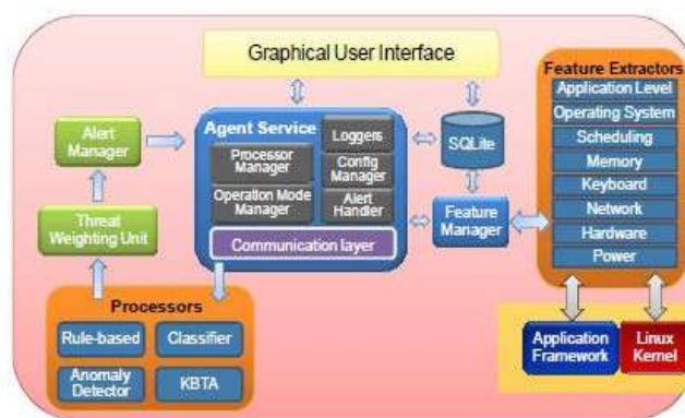
Figure 1: Mobile Malware Detection framework.
